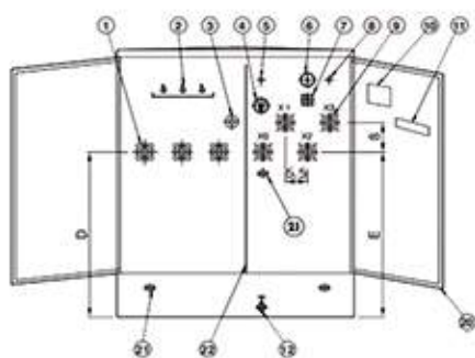
Dead Front Radial Feed
